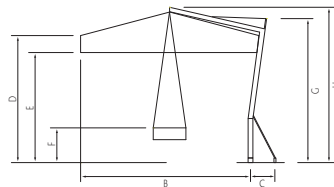
DUO ON GROUND ANCHOR WITH EXTENSION PART
