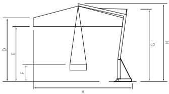
DUO WITH ALUMINIUM BASE
